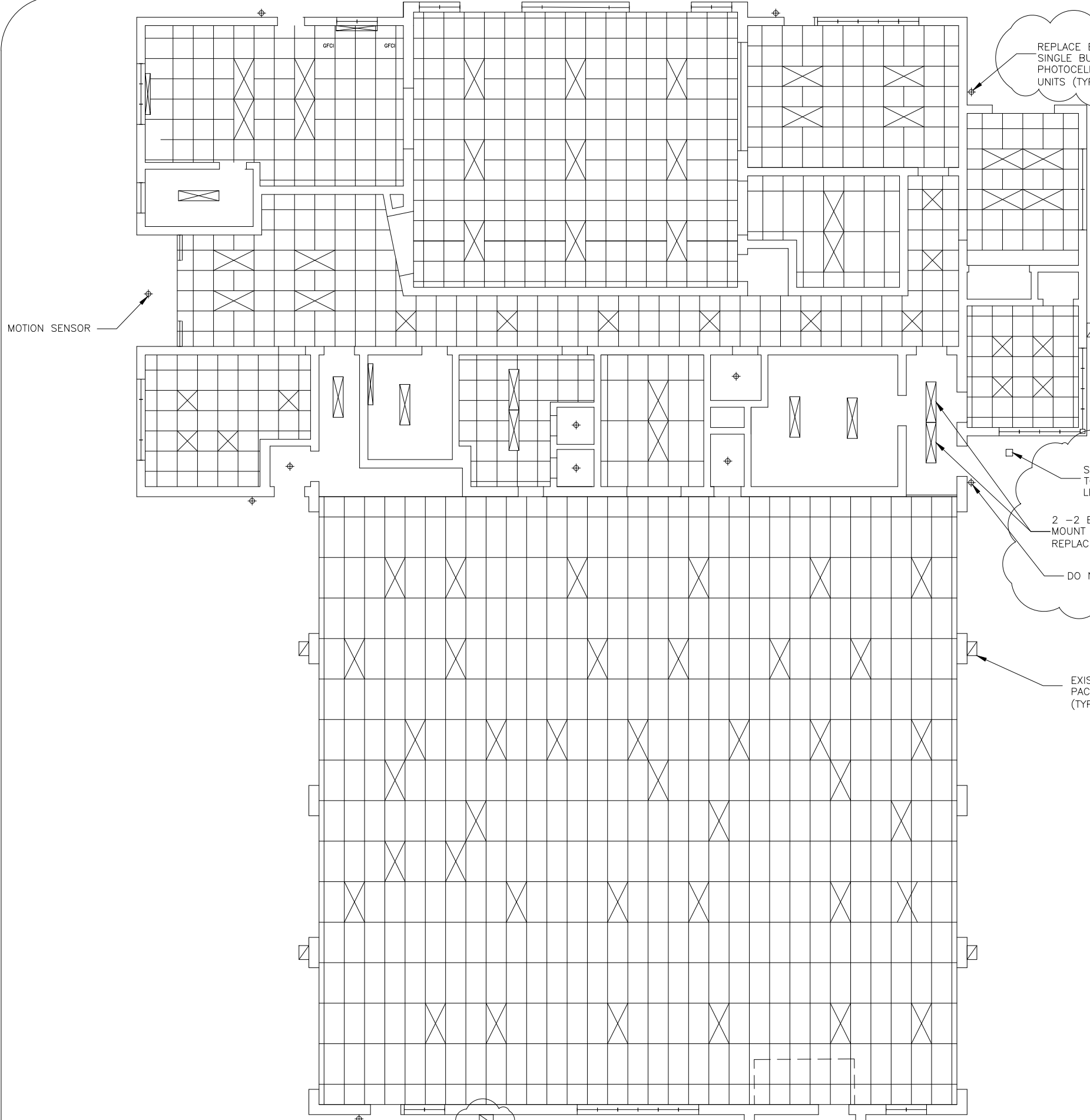
1 Lighting Plan Scale: 3/16"=1'-0"
